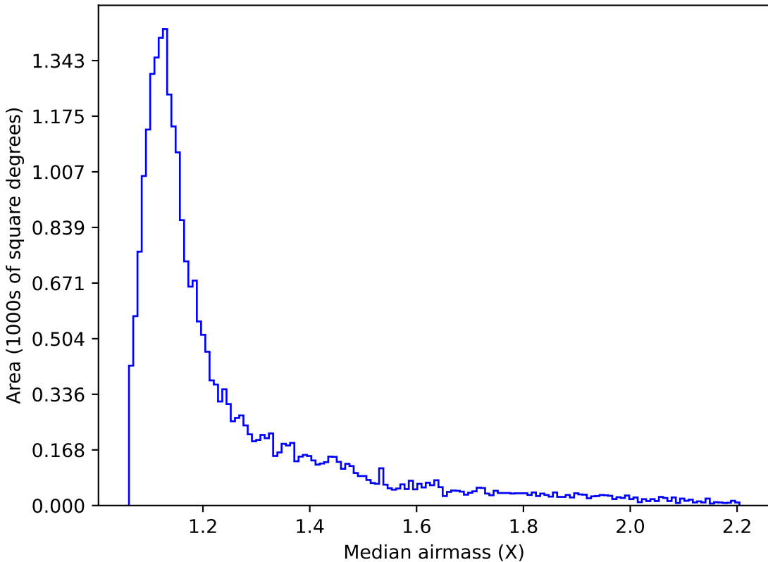
weather_cloudso0v3.5_10yrs Yr 1 r band: Median airmass
