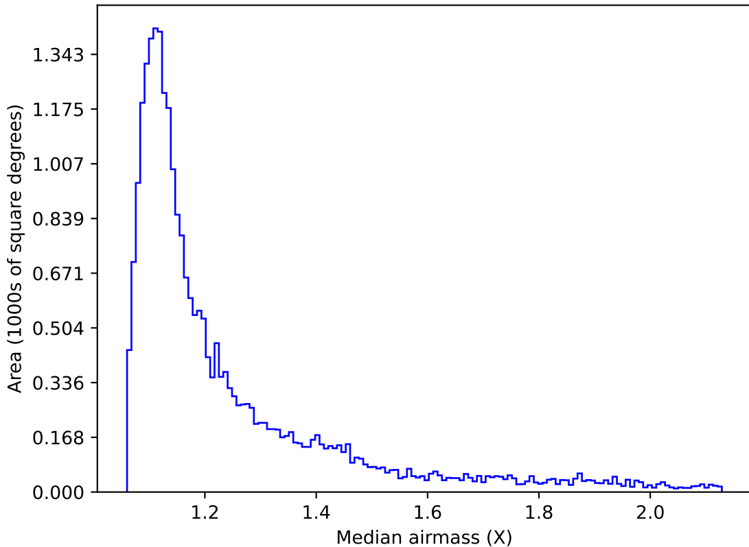
weather_cloudso0v3.5_10yrs Yr 1 i band: Median airmass
