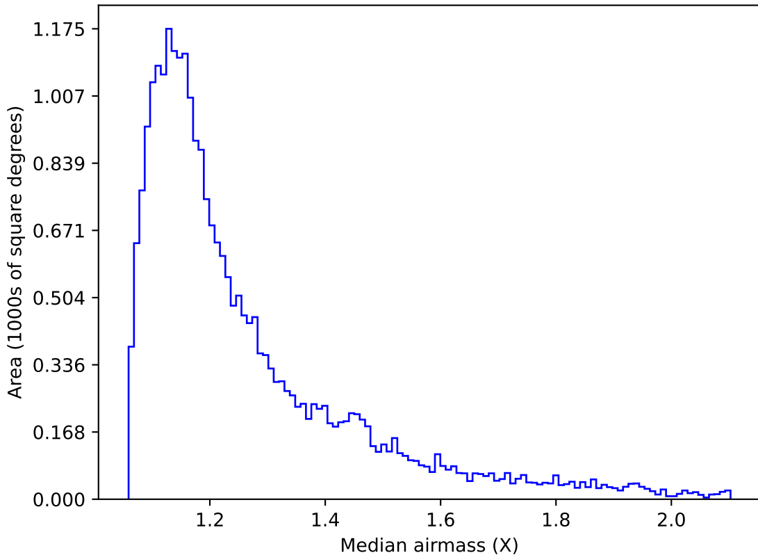
weather_cloudso0v3.5_10yrs Yr 1 g band: Median airmass
