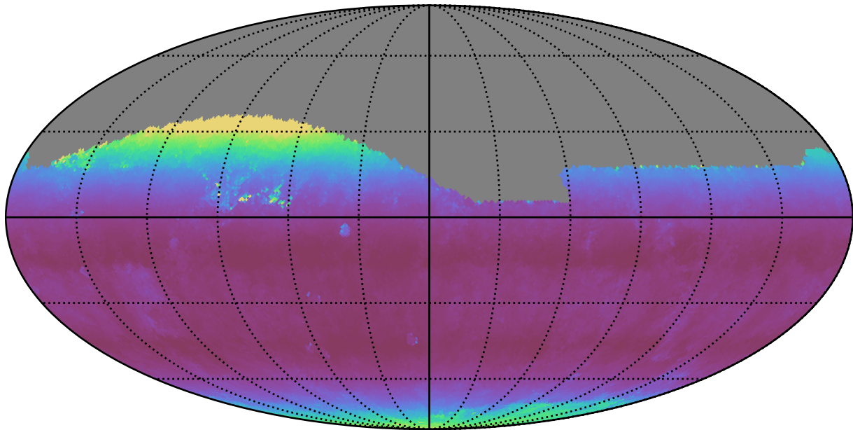
weather_cloudso0v3.5_10yrs Yr 1 all bands: Median airmass
