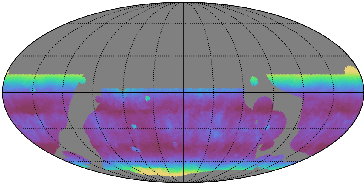
weather_cloudso0v3.5_10yrs WFD z band: Median airmass
