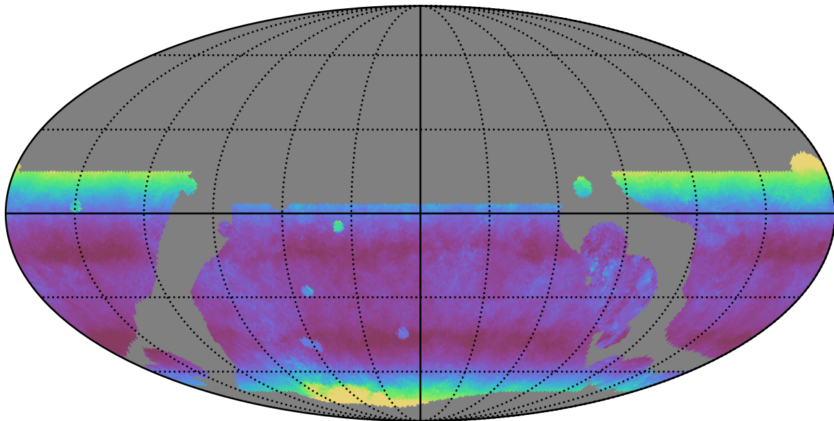
weather_cloudso0v3.5_10yrs WFD y band: Median airmass
