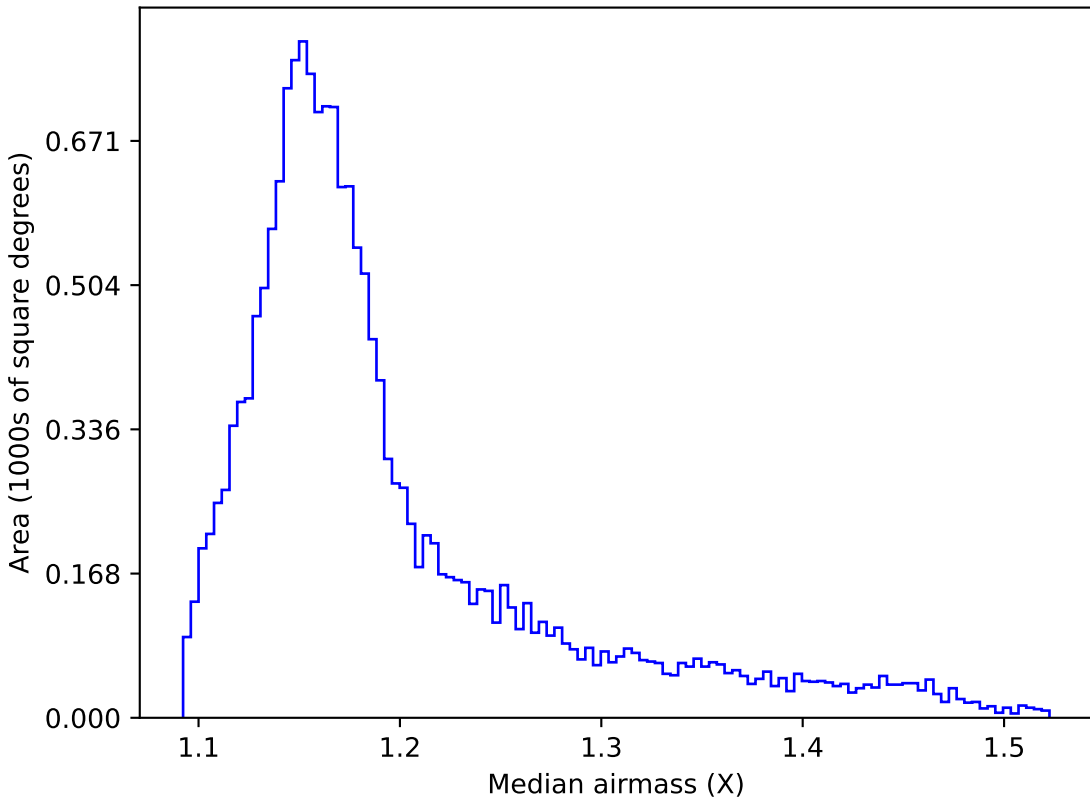
weather_cloudso0v3.5_10yrs WFD y band: Median airmass
