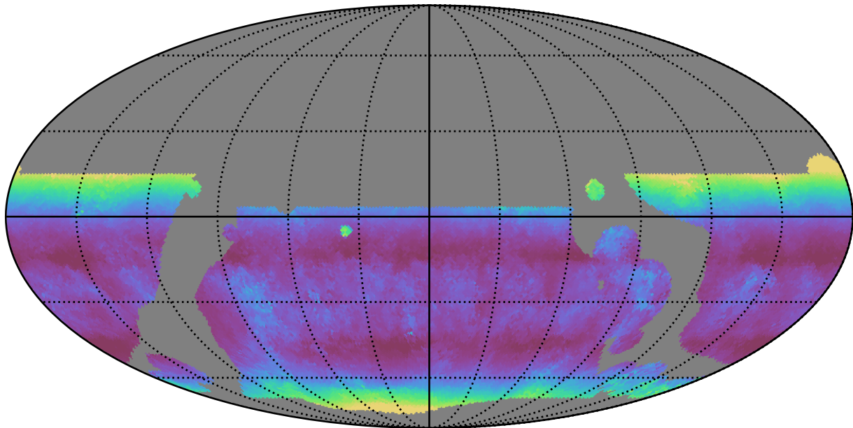
weather_cloudso0v3.5_10yrs WFD u band: Median airmass
