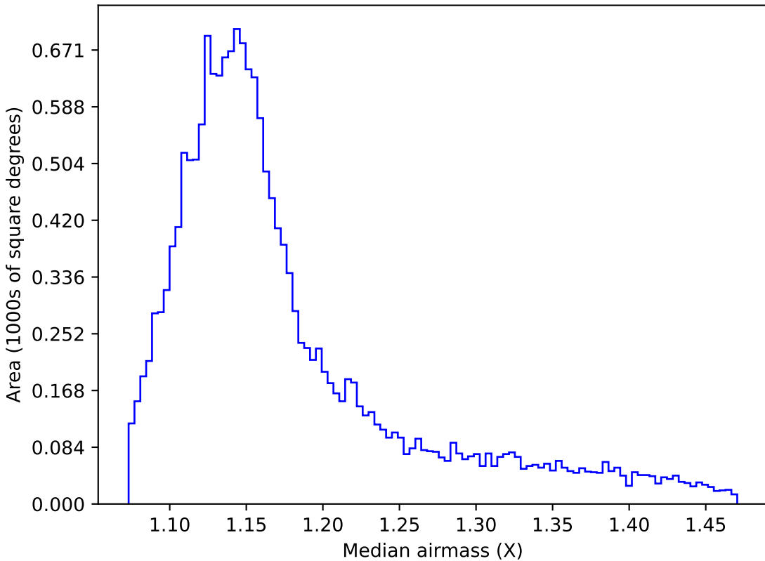
weather_cloudso0v3.5_10yrs WFD u band: Median airmass
