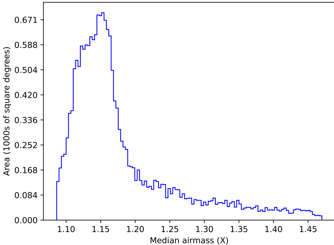
weather_cloudso0v3.5_10yrs WFD i band: Median airmass
