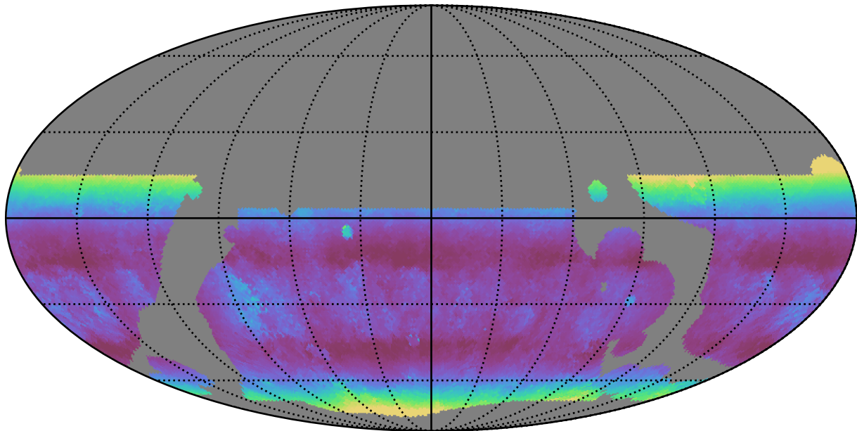
weather_cloudso0v3.5_10yrs WFD g band: Median airmass
