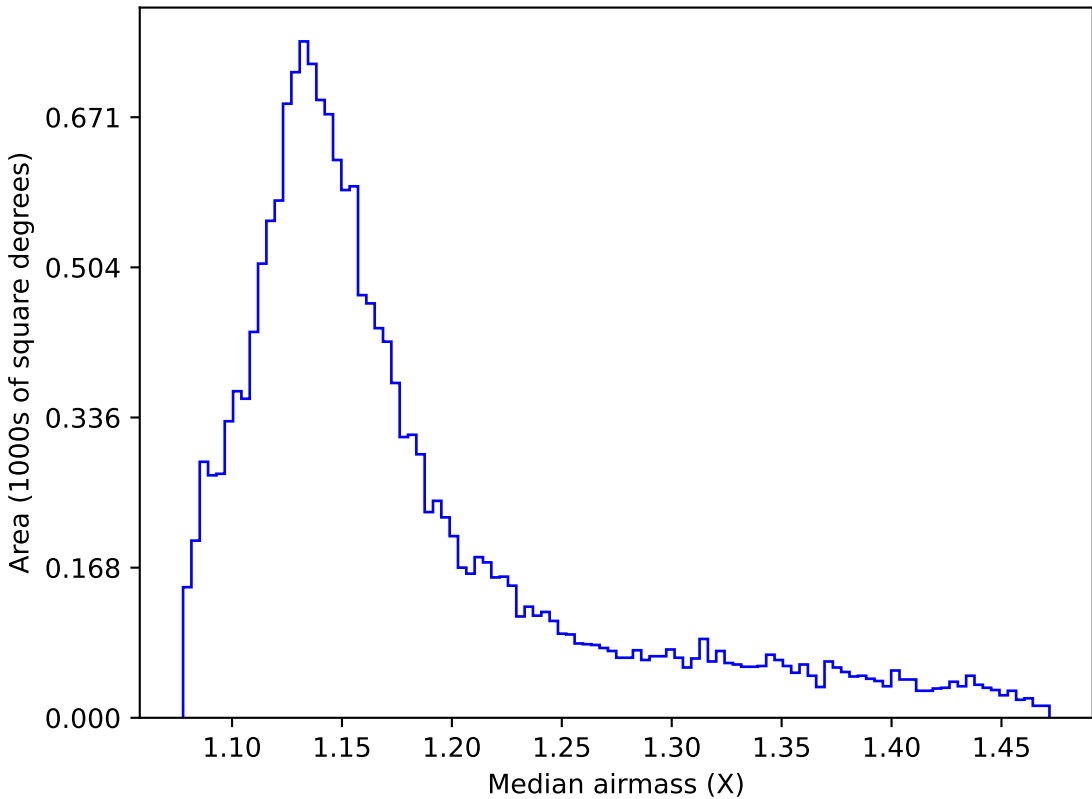
weather_cloudso0v3.5_10yrs WFD g band: Median airmass
