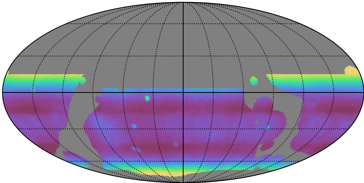
weather_cloudso0v3.5_10yrs WFD all bands: Median airmass
