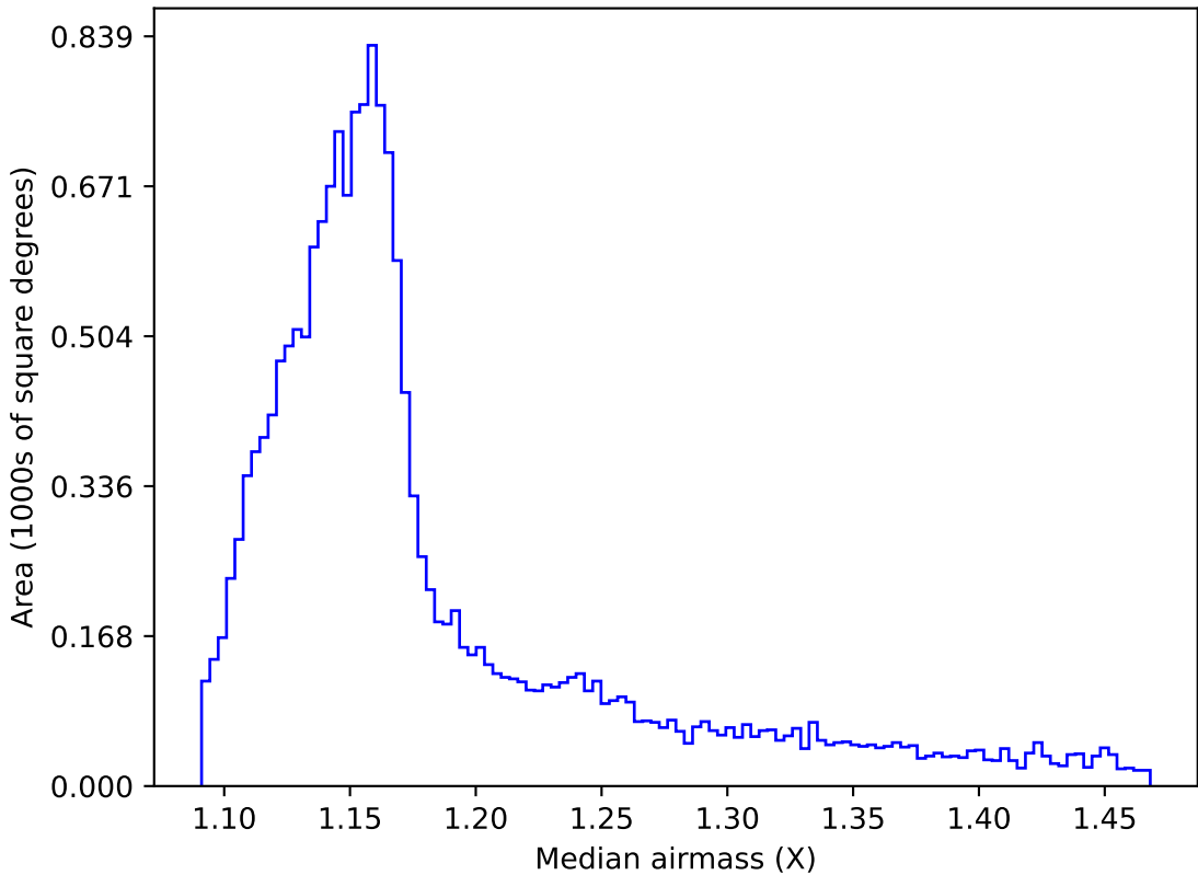
weather_cloudso0v3.5_10yrs WFD all bands: Median airmass
