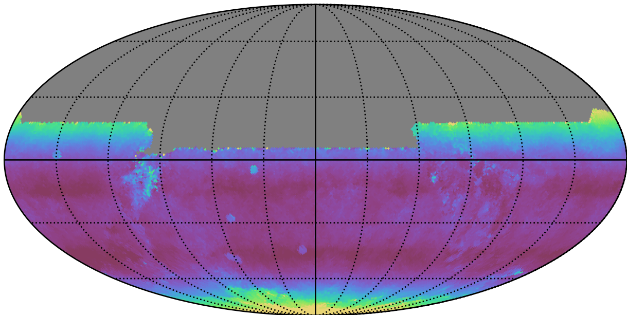
weather_cloudso0v3.5_10yrs All sky y band: Median airmass
