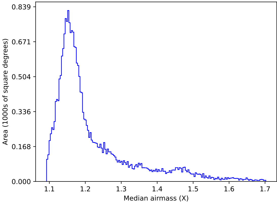
weather_cloudso0v3.5_10yrs All sky y band: Median airmass
