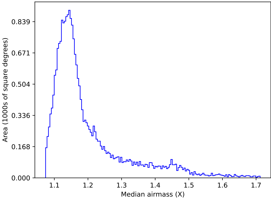
weather_cloudso0v3.5_10yrs All sky u band: Median airmass
