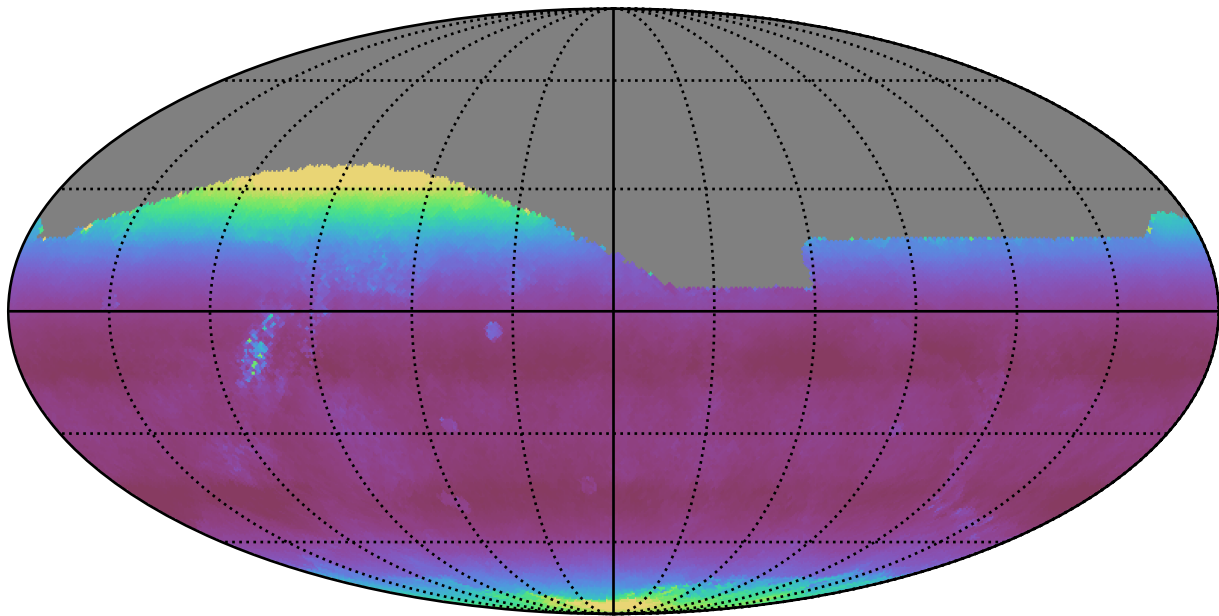
weather_cloudso0v3.5_10yrs All sky r band: Median airmass
