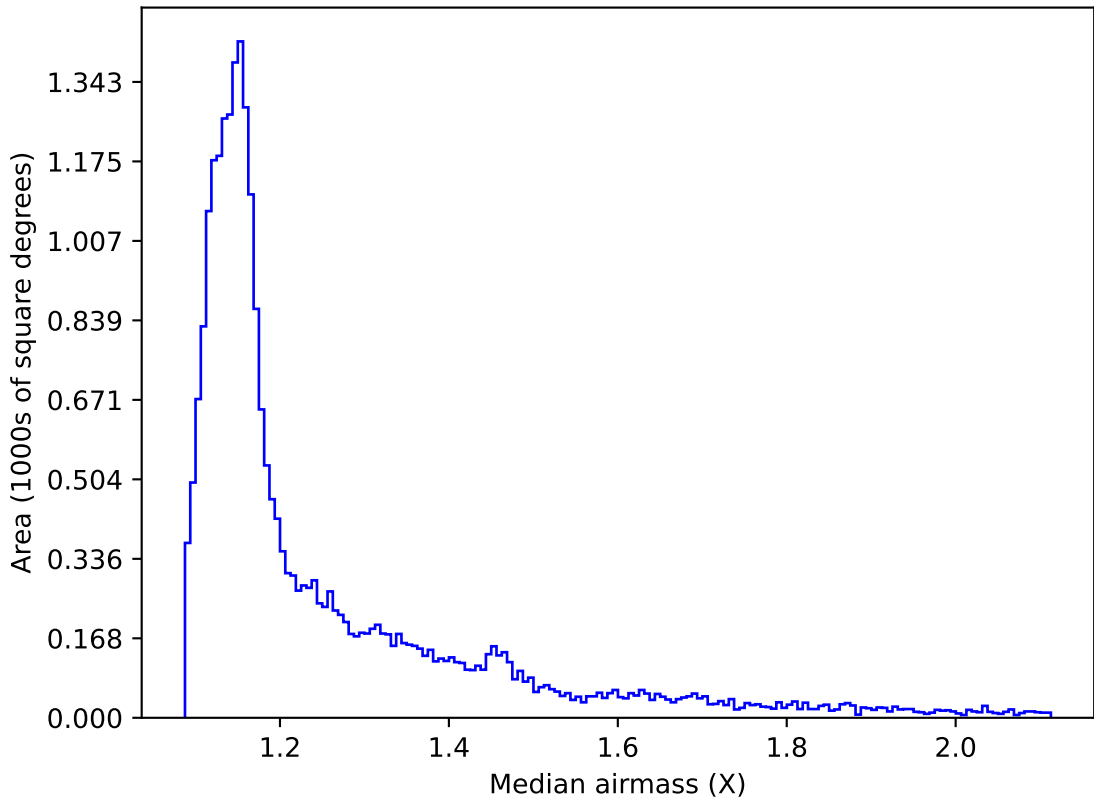
weather_cloudso0v3.5_10yrs All sky i band: Median airmass
