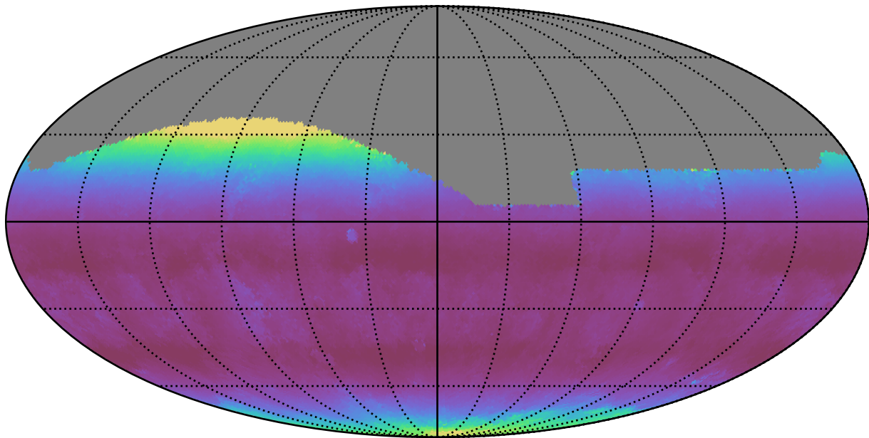
weather_cloudso0v3.5_10yrs All sky g band: Median airmass
