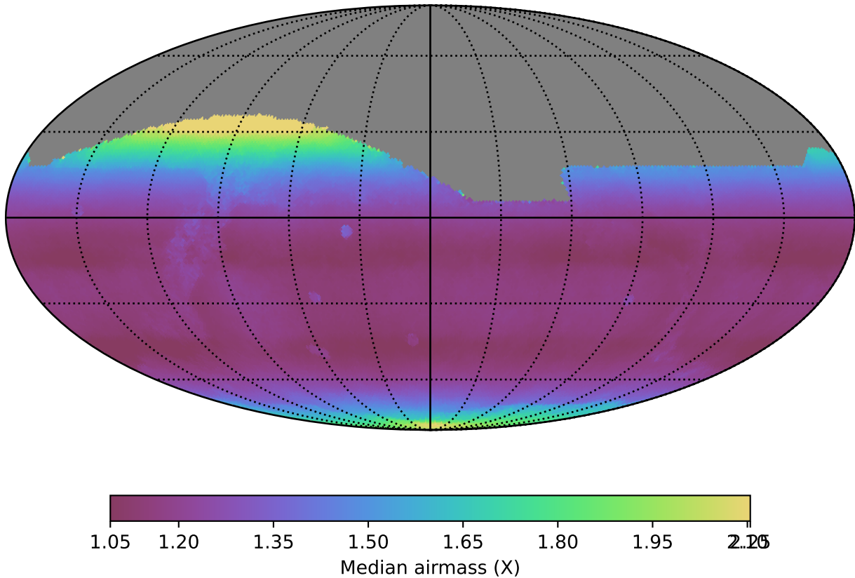
weather_cloudso0v3.5_10yrs All sky all bands: Median airmass
