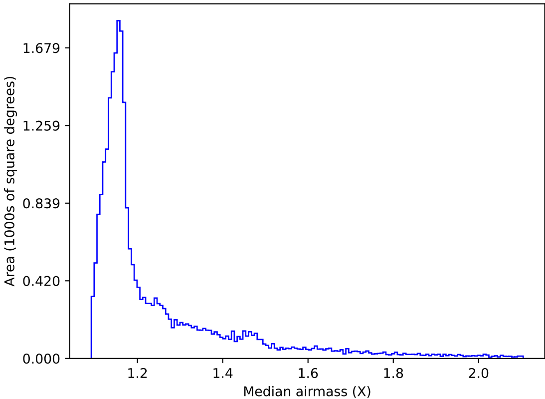
weather_cloudso0v3.5_10yrs All sky all bands: Median airmass
