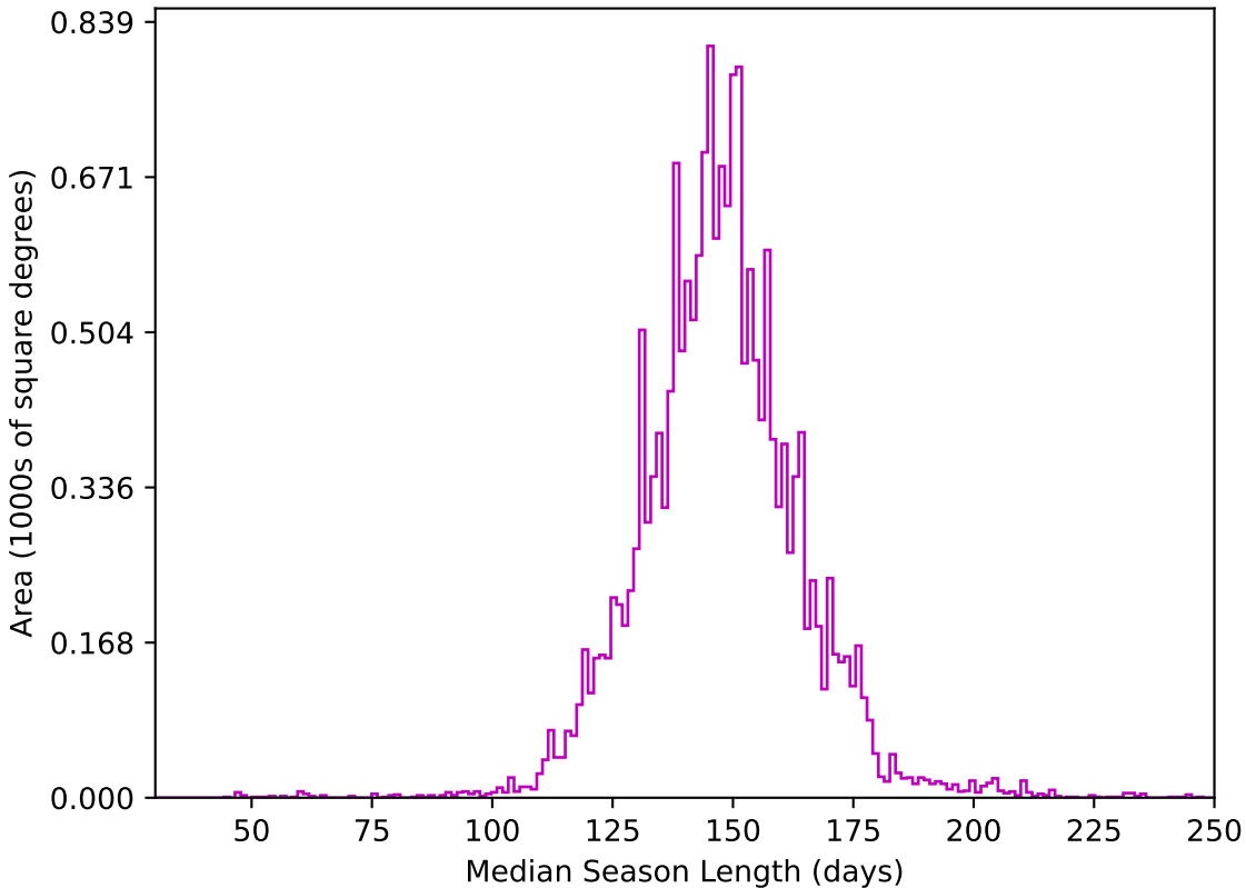
weather_cloudso0v3.5_10yrs WFD z band: Median Season Length
