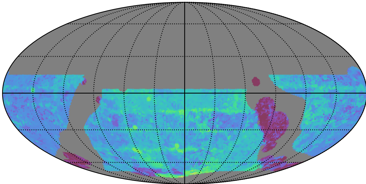
weather_cloudso0v3.5_10yrs WFD y band: Median Season Length
