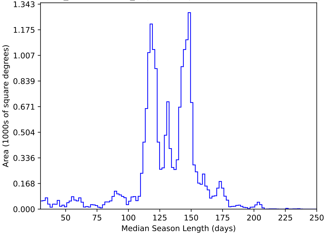
weather_cloudso0v3.5_10yrs WFD y band: Median Season Length
