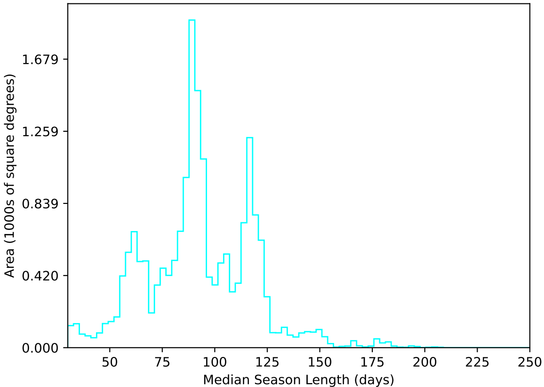
weather_cloudso0v3.5_10yrs WFD u band: Median Season Length
