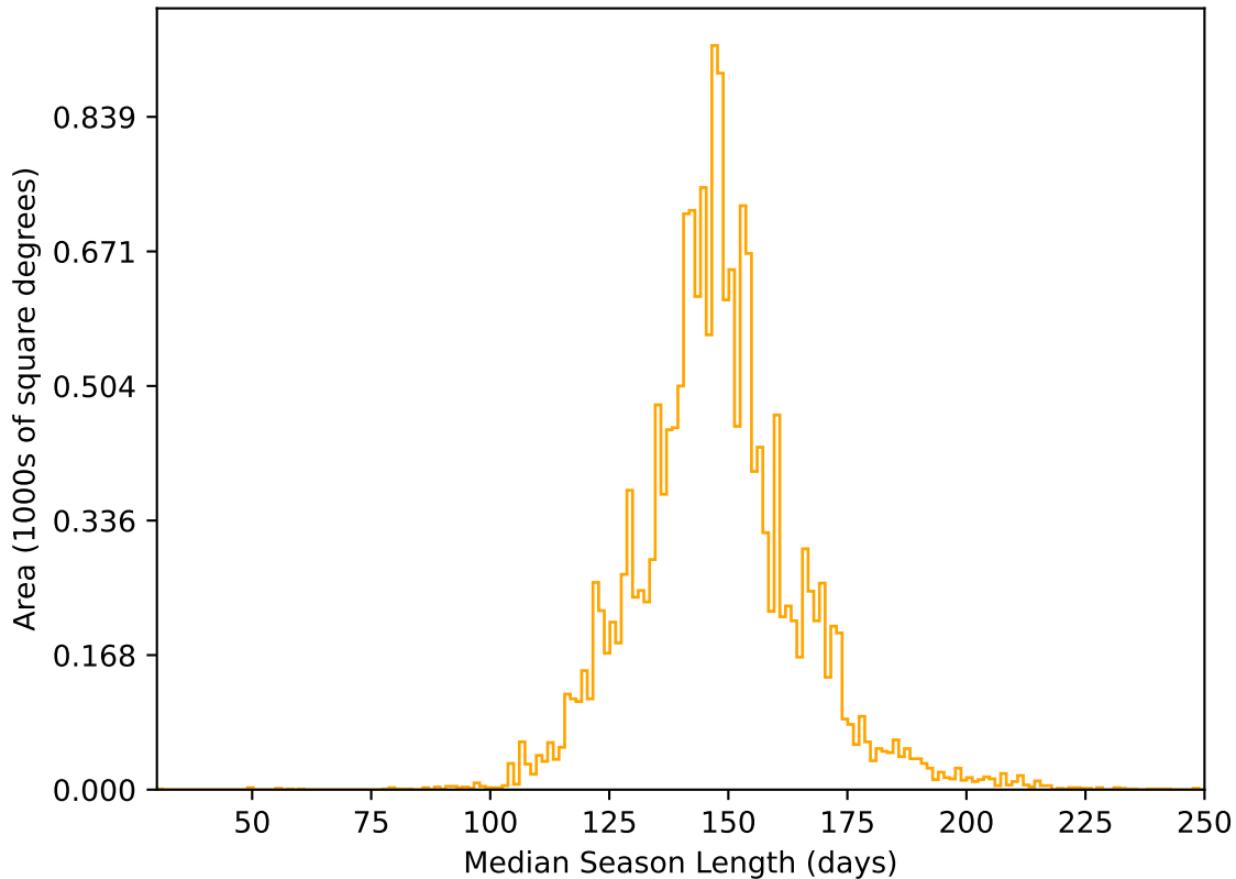
weather_cloudso0v3.5_10yrs WFD r band: Median Season Length
