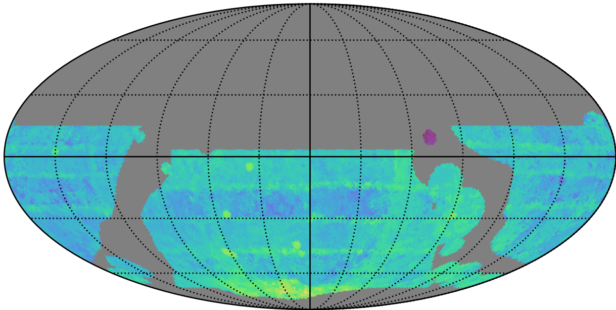
weather_cloudso0v3.5_10yrs WFD i band: Median Season Length
