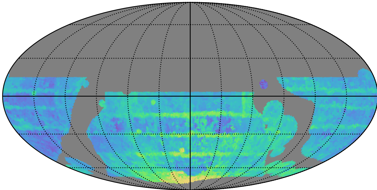
weather_cloudso0v3.5_10yrs WFD all bands: Median Season Length
