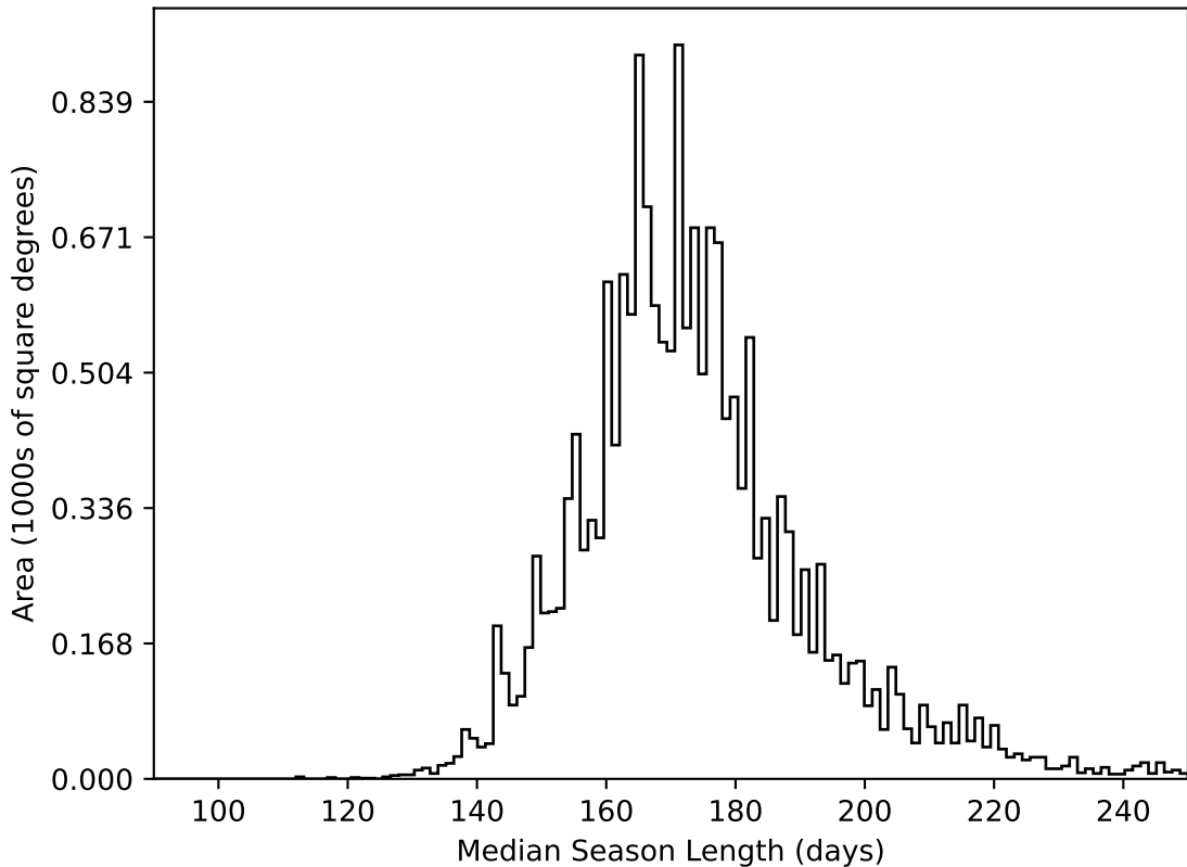
weather_cloudso0v3.5_10yrs WFD all bands: Median Season Length
