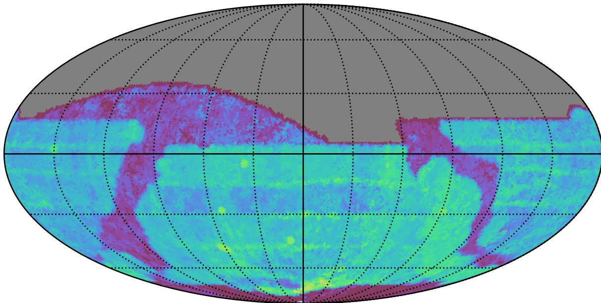
weather_cloudso0v3.5_10yrs All sky z band: Median Season Length
