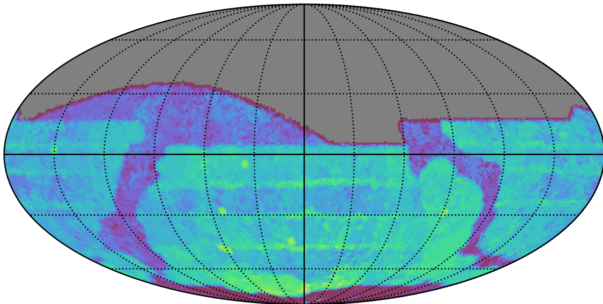
weather_cloudso0v3.5_10yrs All sky r band: Median Season Length
