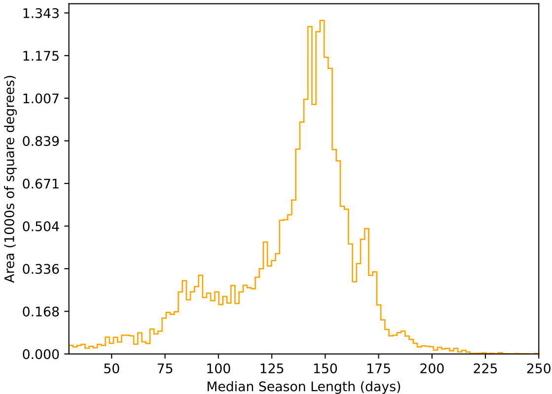
weather_cloudso0v3.5_10yrs All sky r band: Median Season Length
