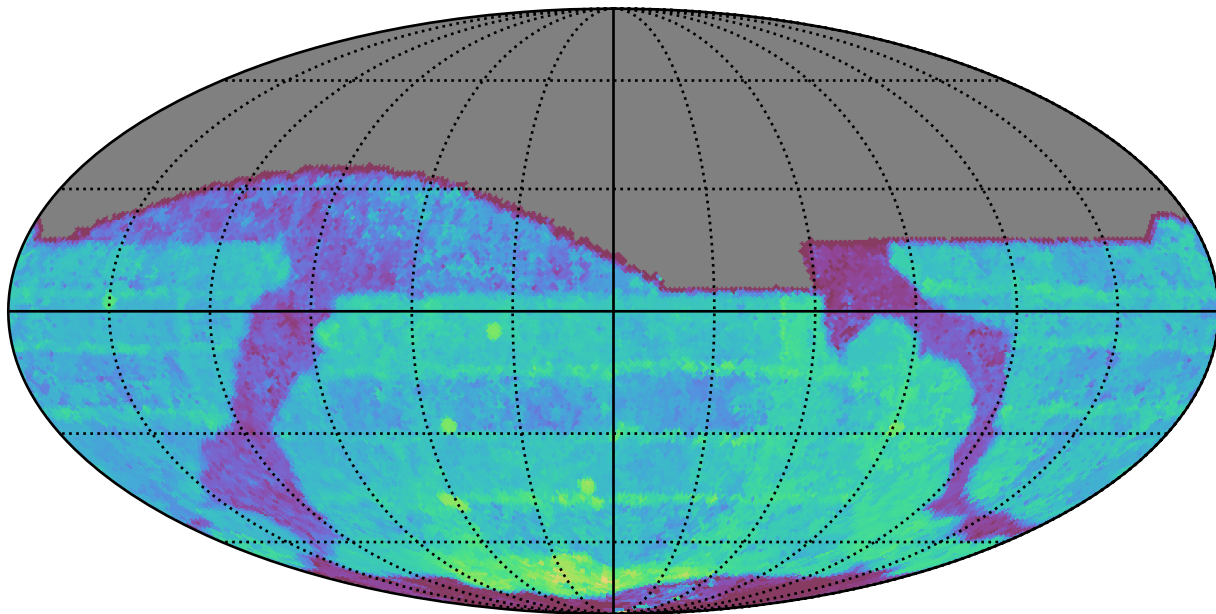
weather_cloudso0v3.5_10yrs All sky i band: Median Season Length
