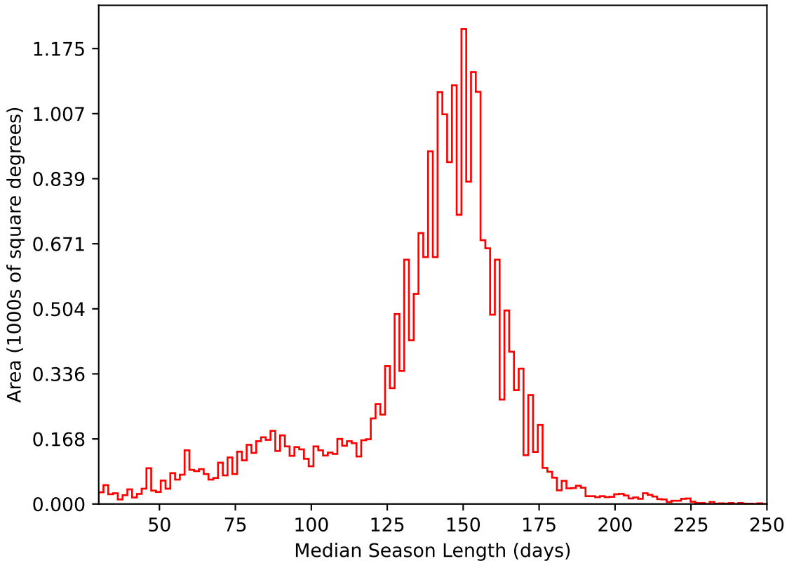
weather_cloudso0v3.5_10yrs All sky i band: Median Season Length
