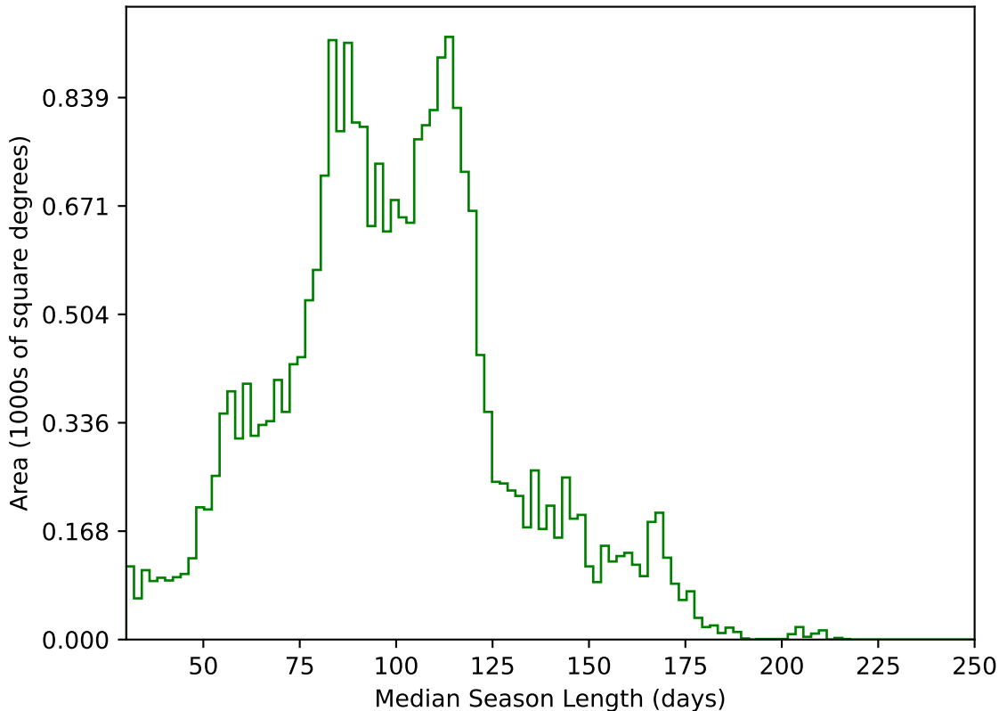
weather_cloudso0v3.5_10yrs All sky g band: Median Season Length
