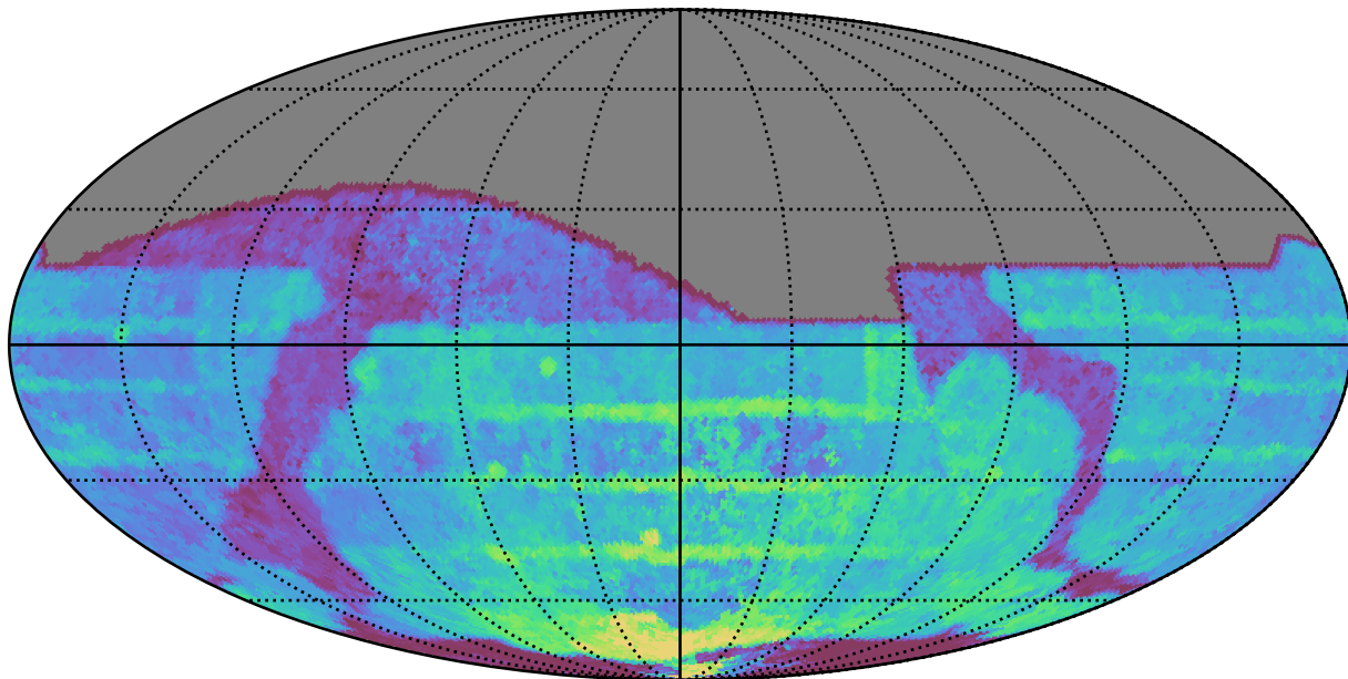
weather_cloudso0v3.5_10yrs All sky all bands: Median Season Length
