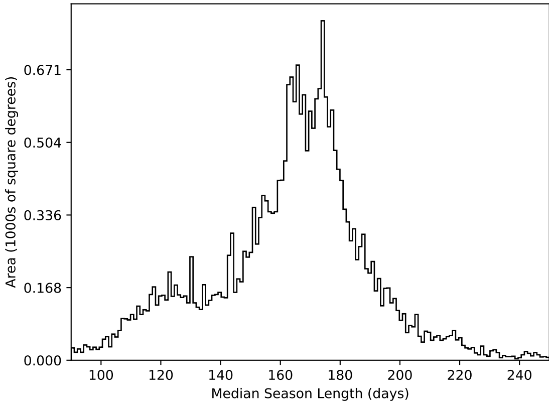
weather_cloudso0v3.5_10yrs All sky all bands: Median Season Length
