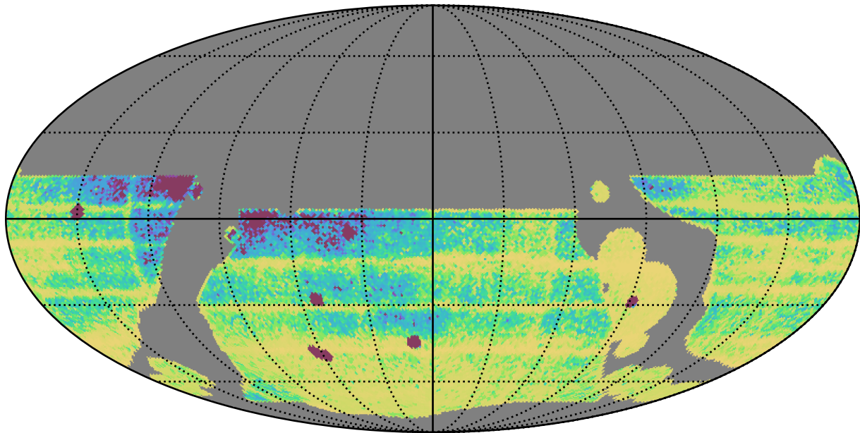
weather_cloudso0v3.5_10yrs WFD: Median Intra-Night Gap
