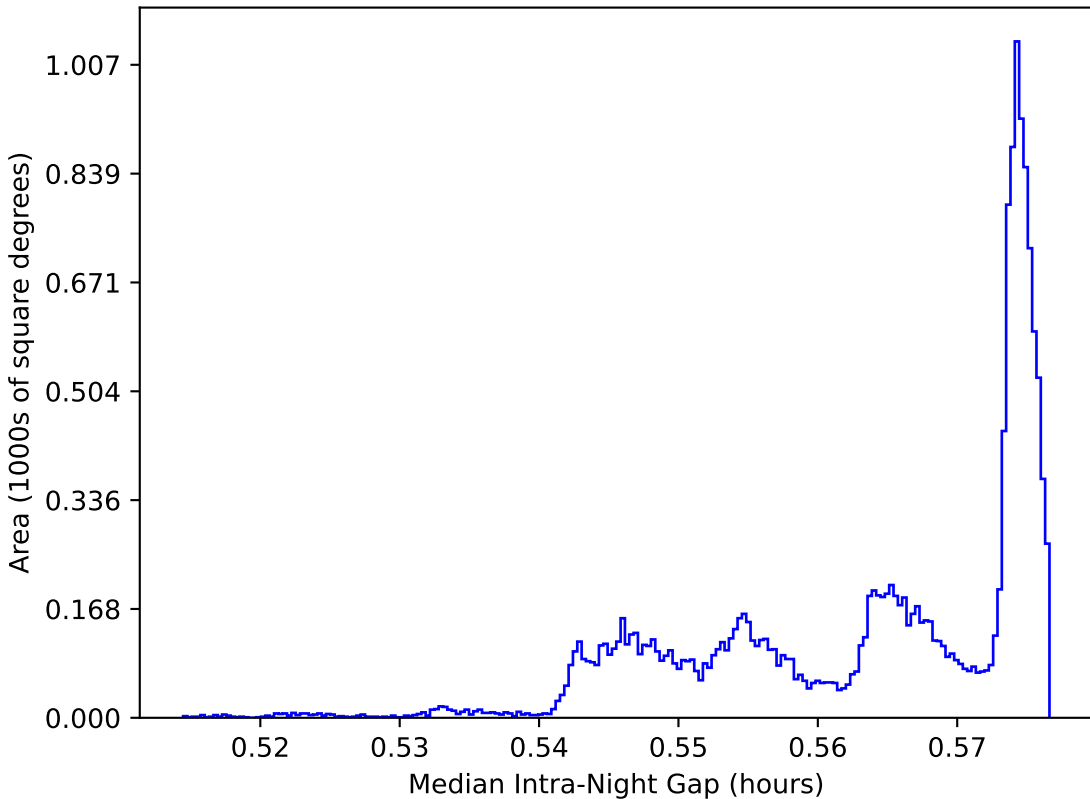
weather_cloudso0v3.5_10yrs WFD: Median Intra-Night Gap
