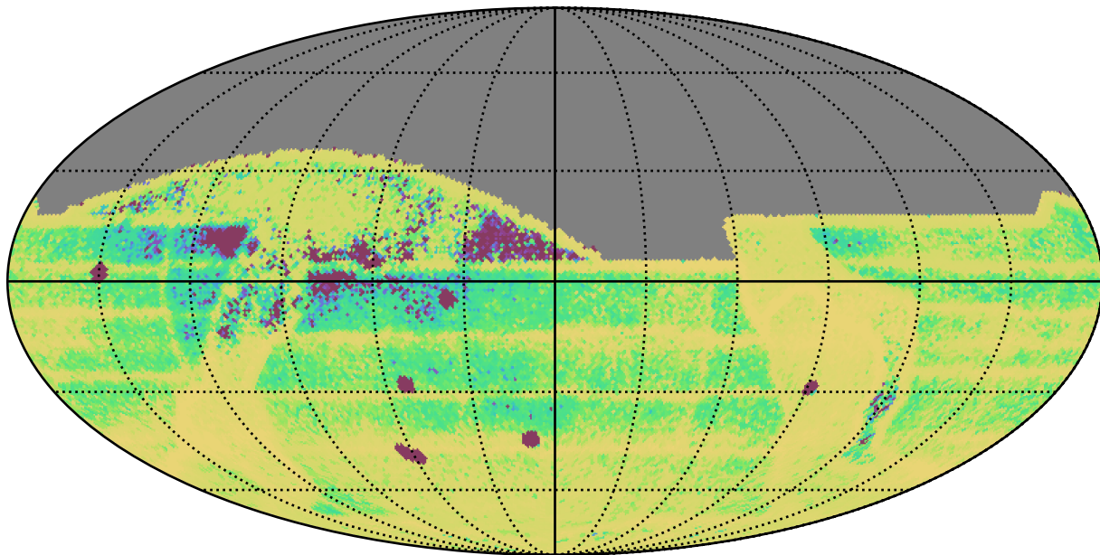
weather_cloudso0v3.5_10yrs All sky: Median Intra-Night Gap
