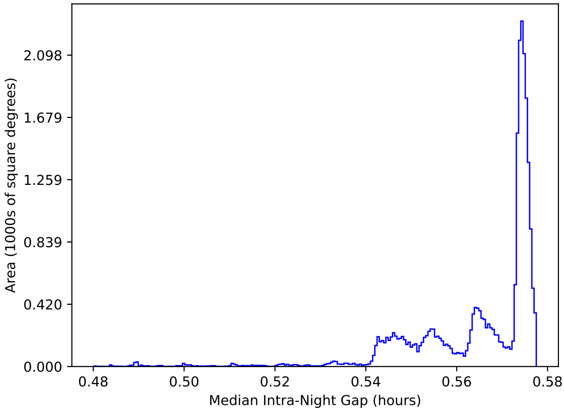
weather_cloudso0v3.5_10yrs All sky: Median Intra-Night Gap
