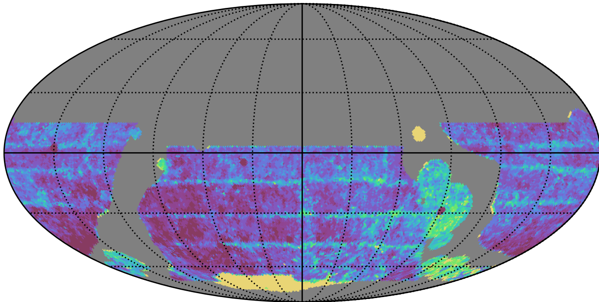
weather_cloudso0v3.5_10yrs WFD z band: Median Inter-Night Gap
