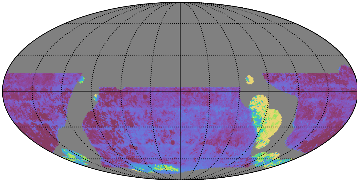
weather_cloudso0v3.5_10yrs WFD y band: Median Inter-Night Gap
