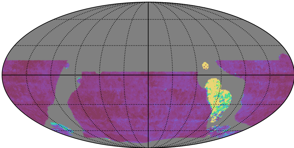
weather_cloudso0v3.5_10yrs WFD u band: Median Inter-Night Gap
