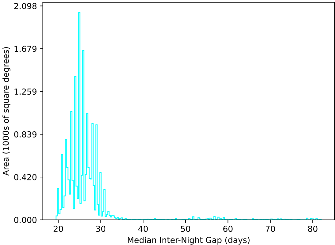
weather_cloudso0v3.5_10yrs WFD u band: Median Inter-Night Gap
