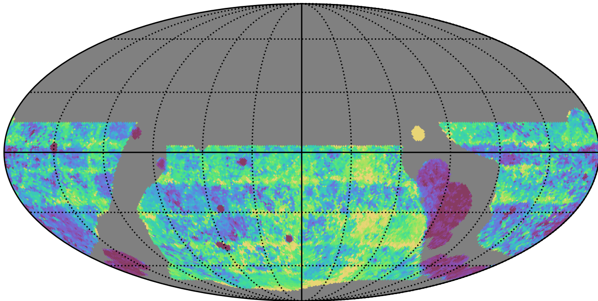
weather_cloudso0v3.5_10yrs WFD g band: Median Inter-Night Gap
