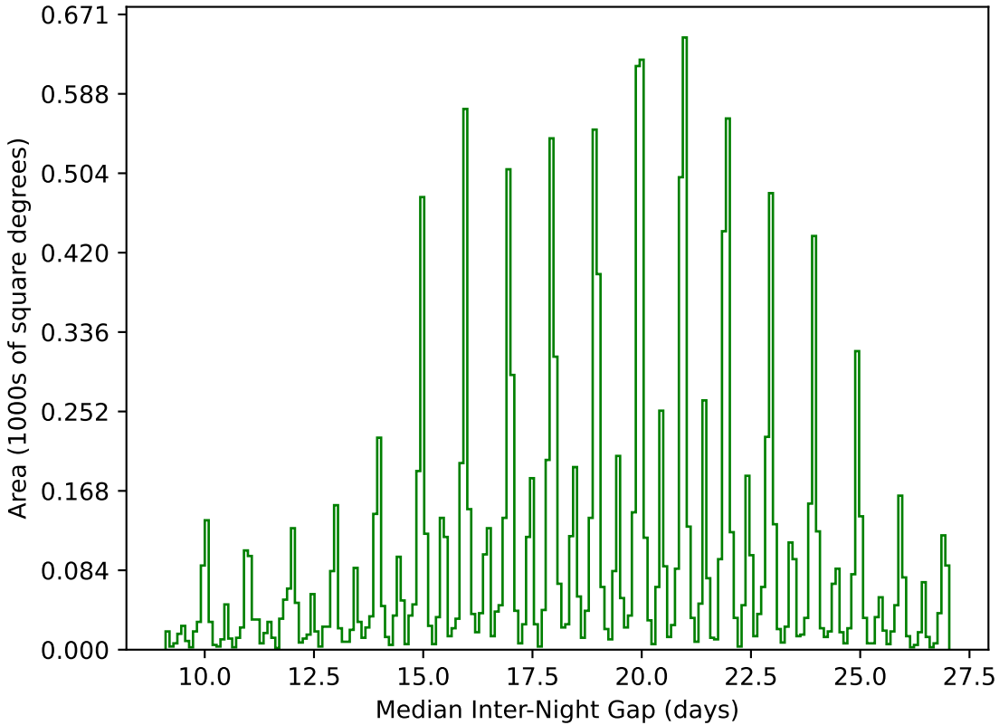
weather_cloudso0v3.5_10yrs WFD g band: Median Inter-Night Gap
