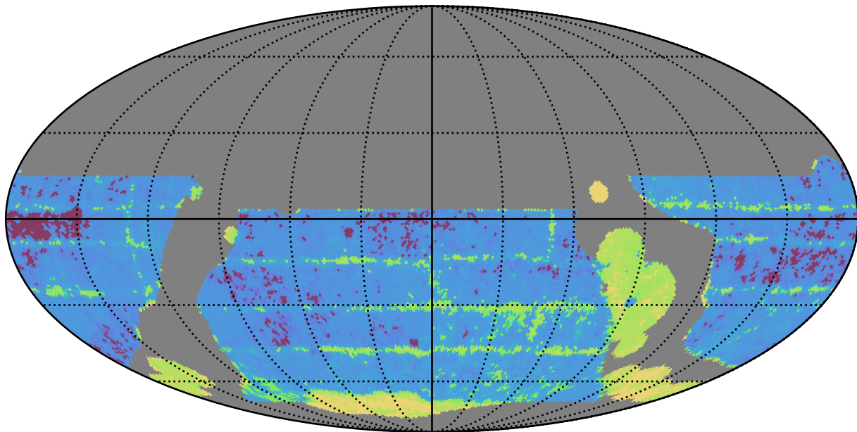
weather_cloudso0v3.5_10yrs WFD all bands: Median Inter-Night Gap
