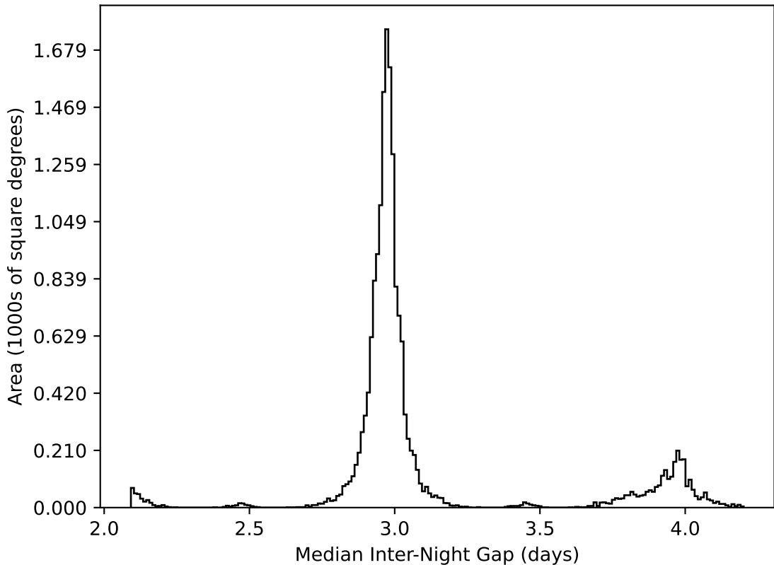
weather_cloudso0v3.5_10yrs WFD all bands: Median Inter-Night Gap
